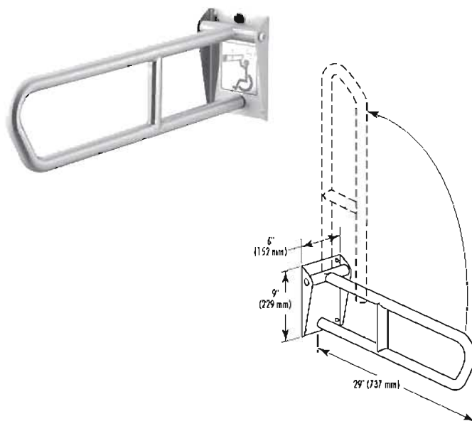
MODEL 8370-101 Bradex®
