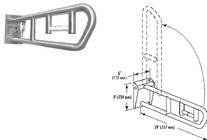
MODEL 8370-103 Bradex®
